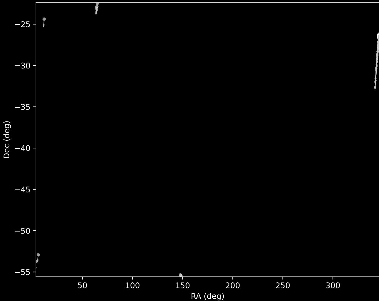
GALAH DR4 Cluster 15 Proper Motion Vectors (n=97)
