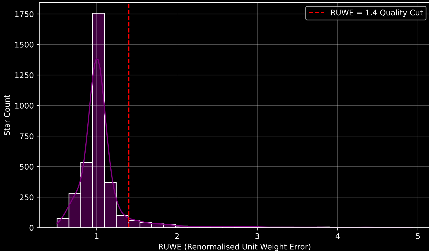
GALAH DR4 Field [-6] RUWE Distribution (n= 3389)
