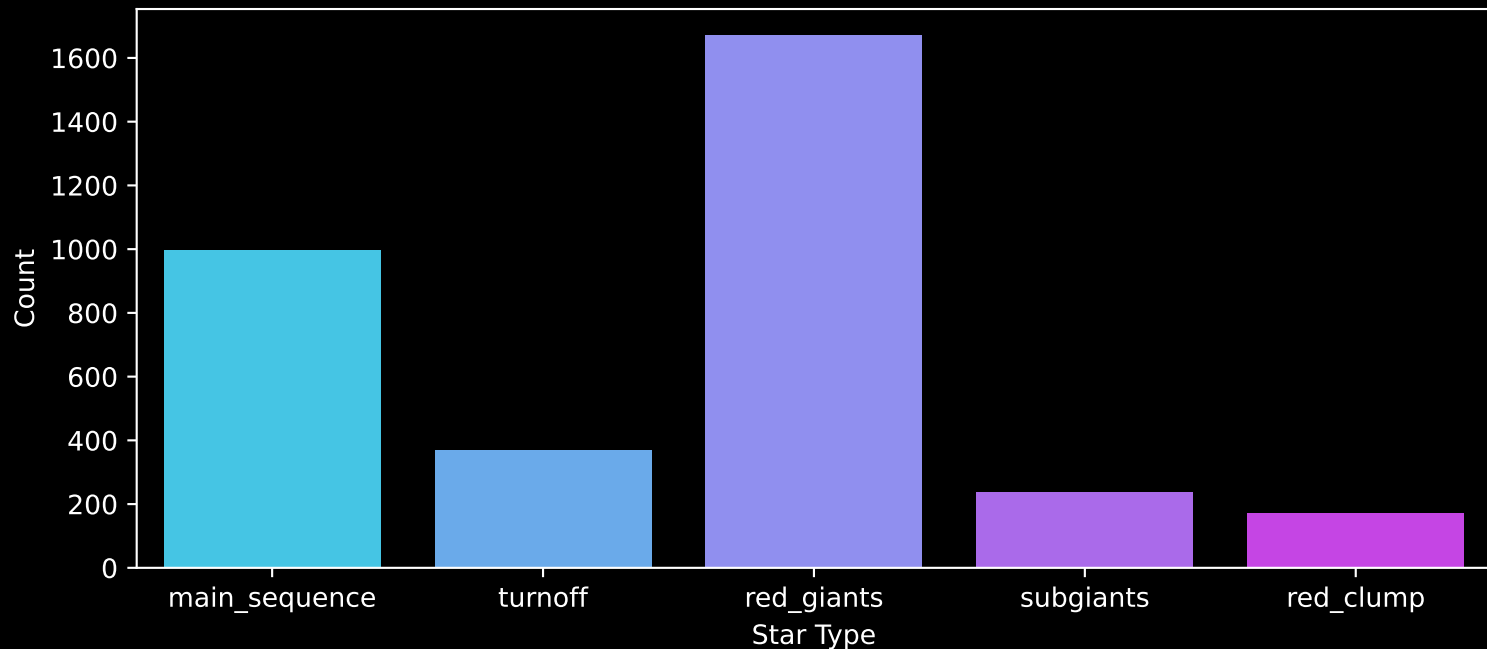
GALAH DR4 Field: [-6] Count plot of Star Type
