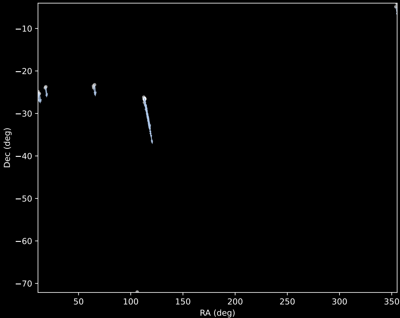
GALAH DR4 Cluster 81 Proper Motion Vectors (n=109)
