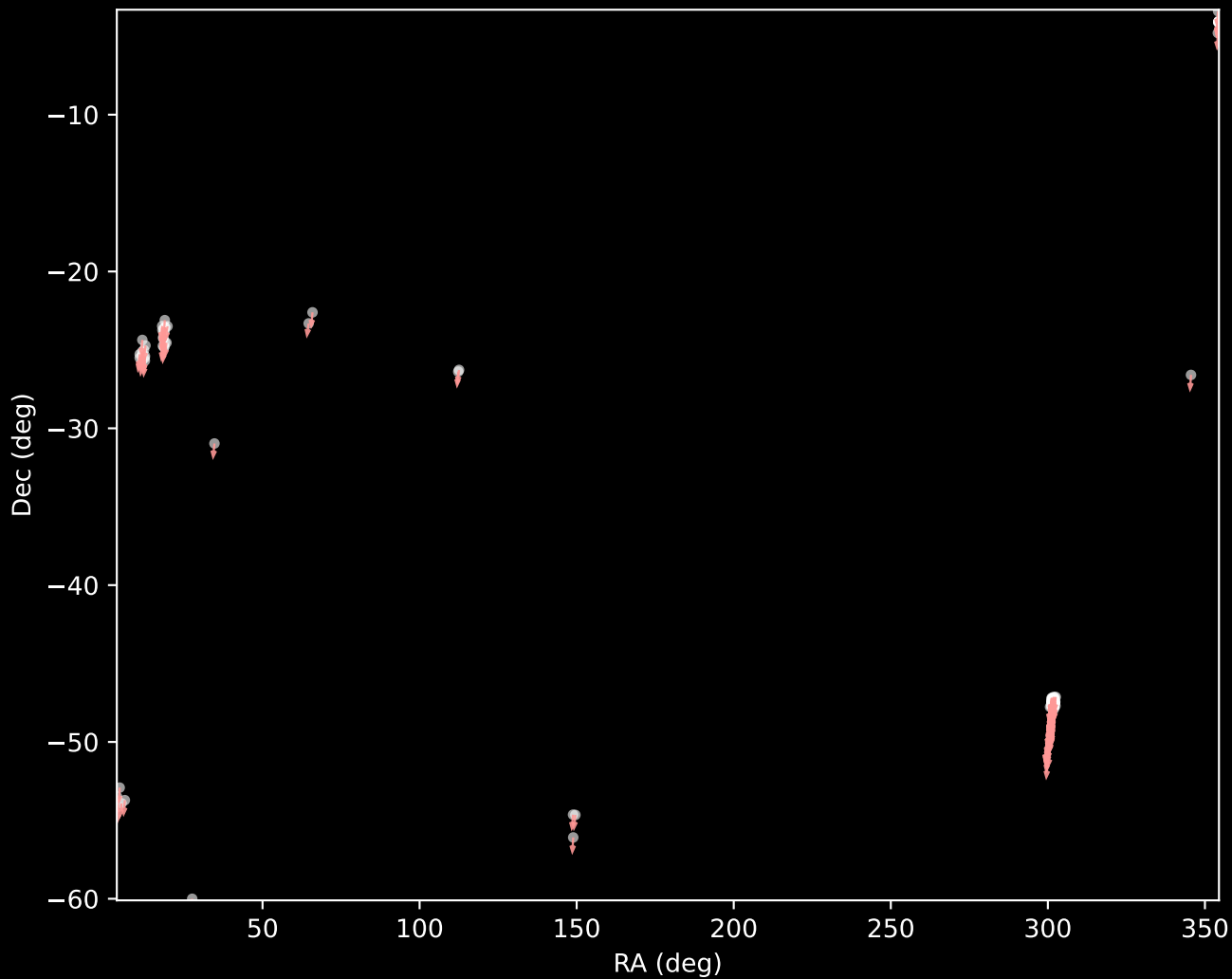
GALAH DR4 Cluster 107 Proper Motion Vectors (n=340)
