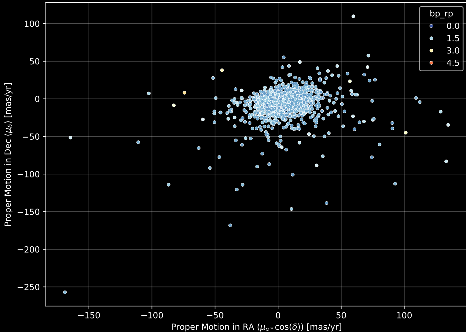
GALAH DR4 Field: [-6] Proper Motion Diagram (n= 3442)
