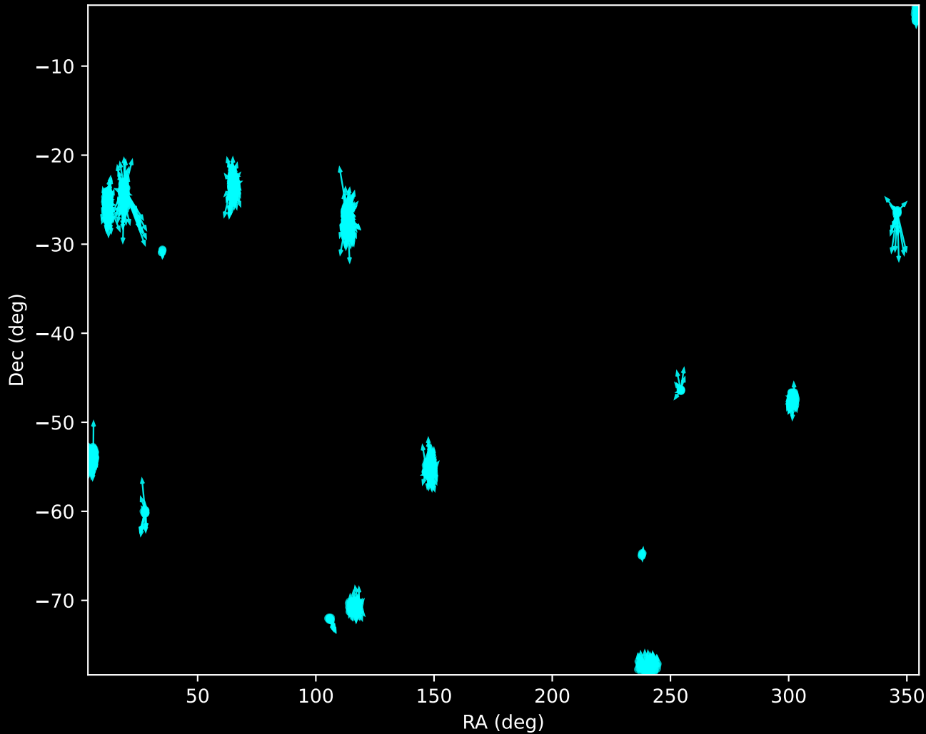
GALAH DR4 Noise Stream Proper Motion Vectors (n=978)
